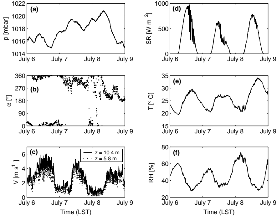
Figure 2. (a) Atmospheric pressure p , (b) wind direction \alpha , (c) horizontal wind speed V measured at two heights, (d) solar radiation SR, (e) air temperature T and (f) relative humidity RH at the Ponca St. field site in Baltimore during July 6–8, 2002. Tick marks along the abscissa axis denote midnight.
